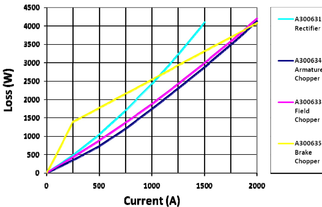
Heatsink Losses
